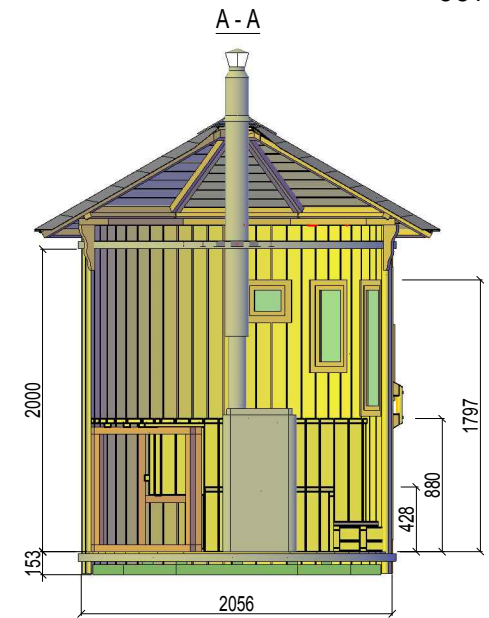
CUT VIEW
