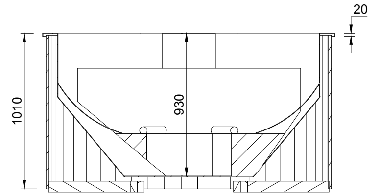
CUT VIEW A-A
